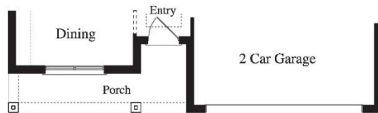
FLOOR PLAN D
