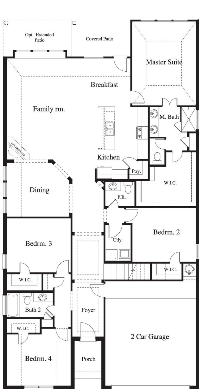
FIRST FLOOR PLAN B&C
